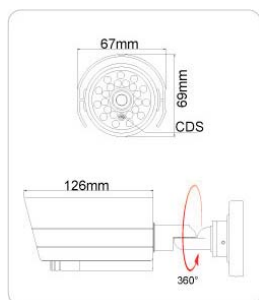
Weatherproof IR camera with 3-Axis bracket IR Distance 20 M
